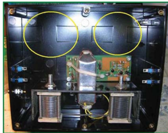
Plate capacitor tuners, silver Sephorah radio coil and solid state amplification visible pre-wiring. Yellow circles show approximate location of input and output wells.
